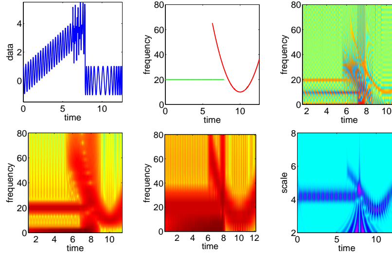
Figure 1. Examples of time-frequency representations. Top row left: the signal f(t) = f_1(t) + f_2(t) defined by f_1(t) = .5t + \cos(20t) for 0 \leq t \leq 5\pi/2 , and f_2(t) = \cos(\frac{4}{3}[(t-10)^3 - (2\pi-10)^3] + 10(t-2\pi)) for 2\pi \leq t \leq 4\pi ; middle: the “instantaneous frequency” for its two components: for f_1 , \omega(t) = 20 for 0 \leq (t-10)^2 \leq 5\pi/2 , and for f_2 , \omega(t) = 4t^2 + 10 for 2\pi \leq t \leq 4\pi ; right: the Wigner-Ville distribution of f . Bottom row left: the (absolute value of a) continuous windowed Fourier transform of f(t) , with a window w_{\text{wide}} with a wide (compact) support in t ; middle: same, but now with a window w_{\text{narrow}} with a less wide (compact) support in t ; right: the (absolute value of a) continuous wavelet transform of f(t) , where \psi is the Morlet wavelet (essentially a modulated Gaussian).
