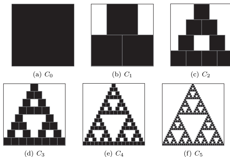
Figure 4. C_0 and the first five iterations C_1-C_5 .
