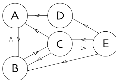
Figure 6. A simple web.
