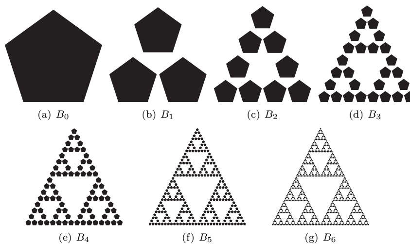
Figure 5. A pentagon B_0 and its first six iterates B_1-B_6 .
