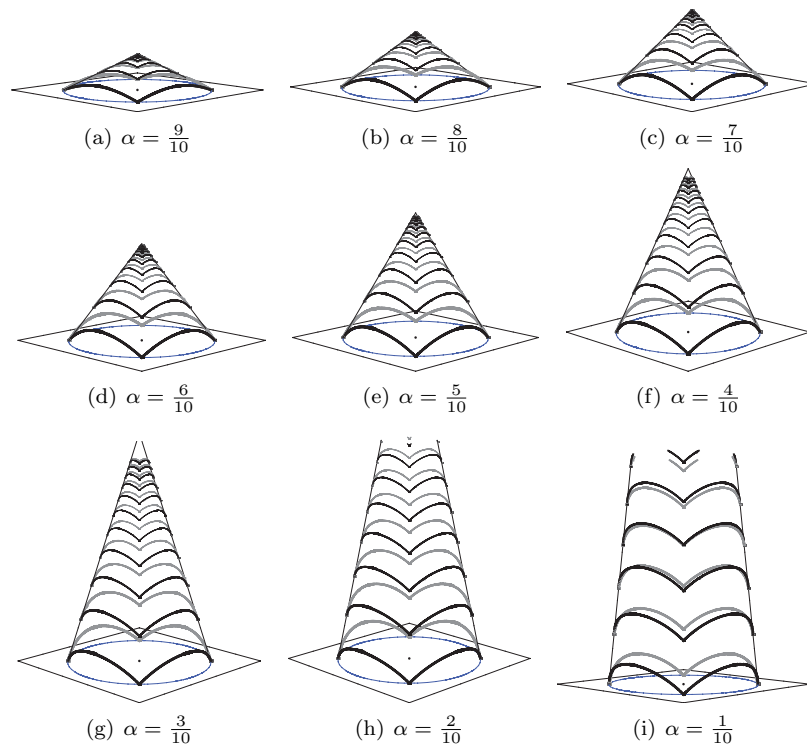
Figure 9. Lifting the image by the center. (Note: the parameter \alpha refers to the transformation \omega(z, \alpha) used to produce the figure and discussed in (1).)
