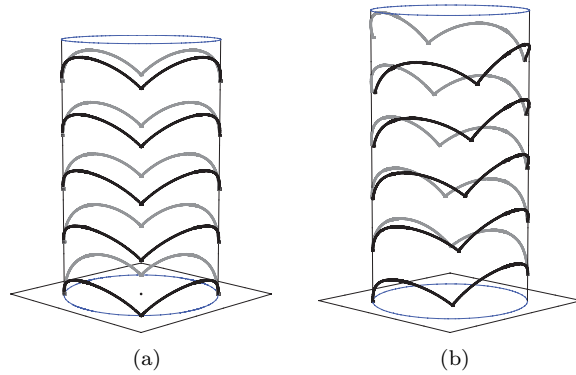
Figure 11. The same images on the cylinder as in Figure 10, with the horizontal plane represented.
